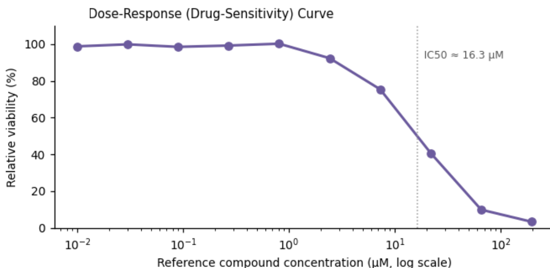
Figure 3. Functional assay readout — IC50 ≈ 16.3 µM.
