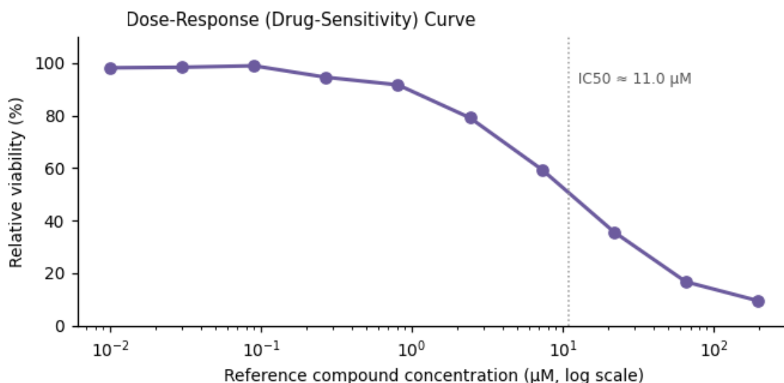
Figure 3. Functional assay readout — IC 50 ≈ 11.0 μM.
