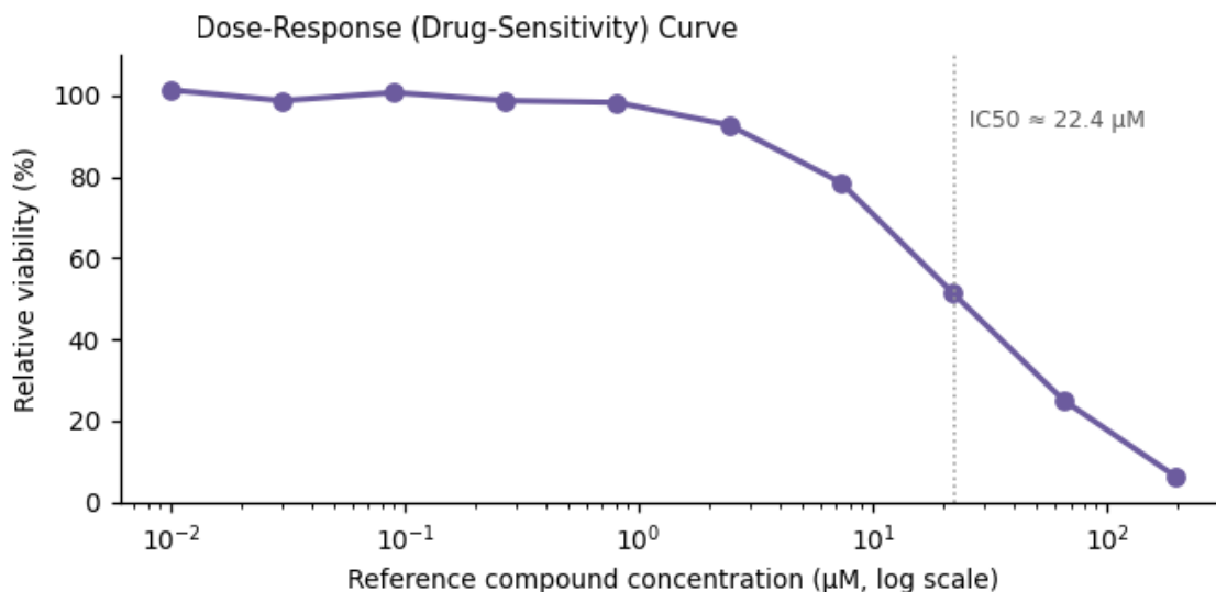
Figure 3. Functional assay readout — IC 50 ≈ 22.4 μM.
