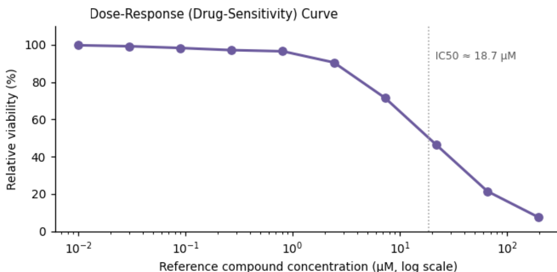
Figure 3. Functional assay readout — IC 50 ≈ 18.7 μM.
