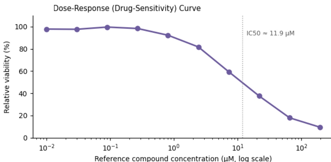
Figure 3. Functional assay readout — IC 50 ≈ 11.9 μM.
