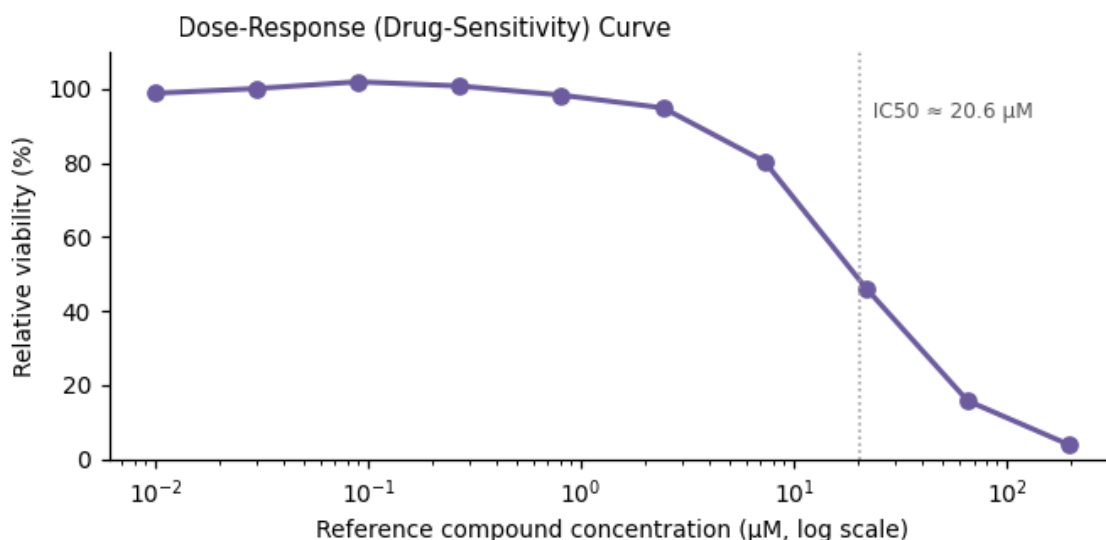
Figure 3. Functional assay readout — IC 50 ≈ 20.6 μM.
