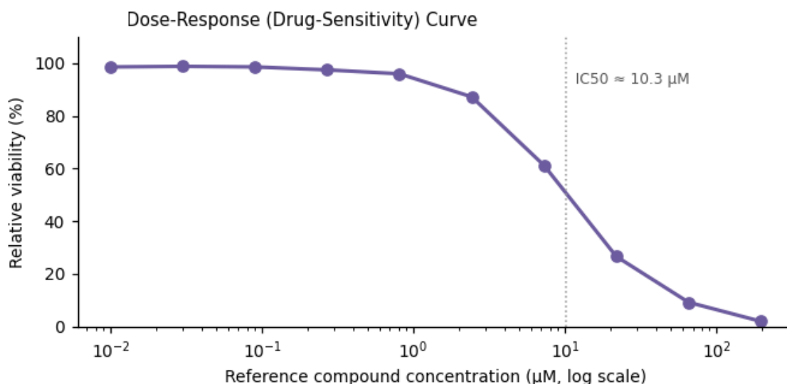
Figure 3. Functional assay readout — IC 50 ≈ 10.3 μM.
