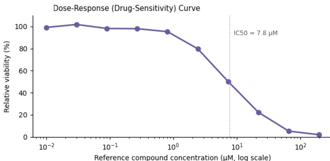
Figure 3. Functional assay readout — IC 50 ≈ 7.8 μM.
