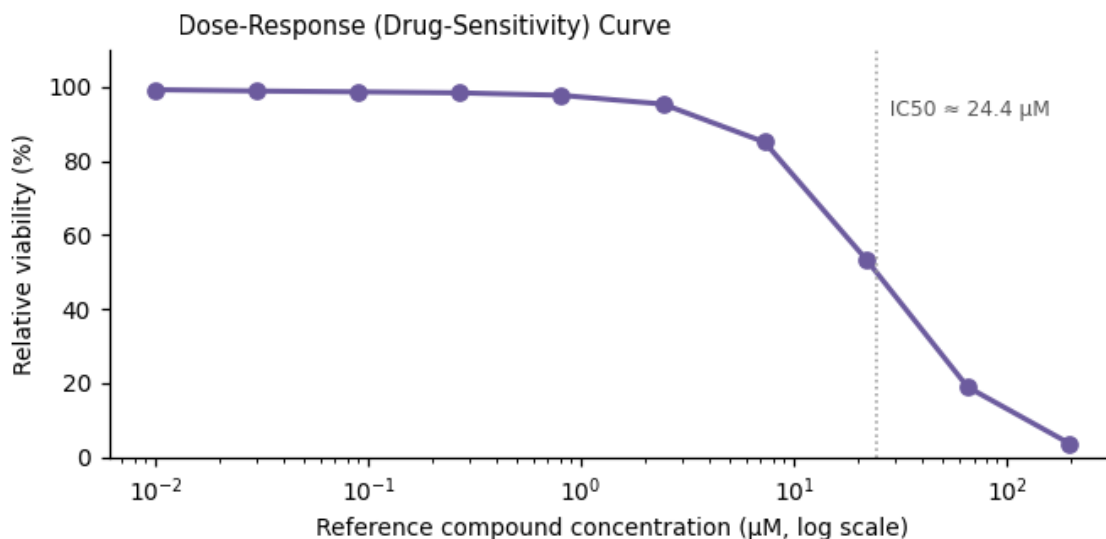
Figure 3. Functional assay readout — IC 50 ≈ 24.4 μM.
