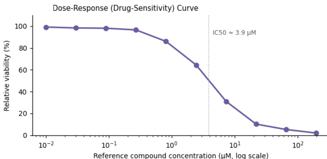
Figure 3. Functional assay readout — IC 50 ≈ 3.9 μM.
