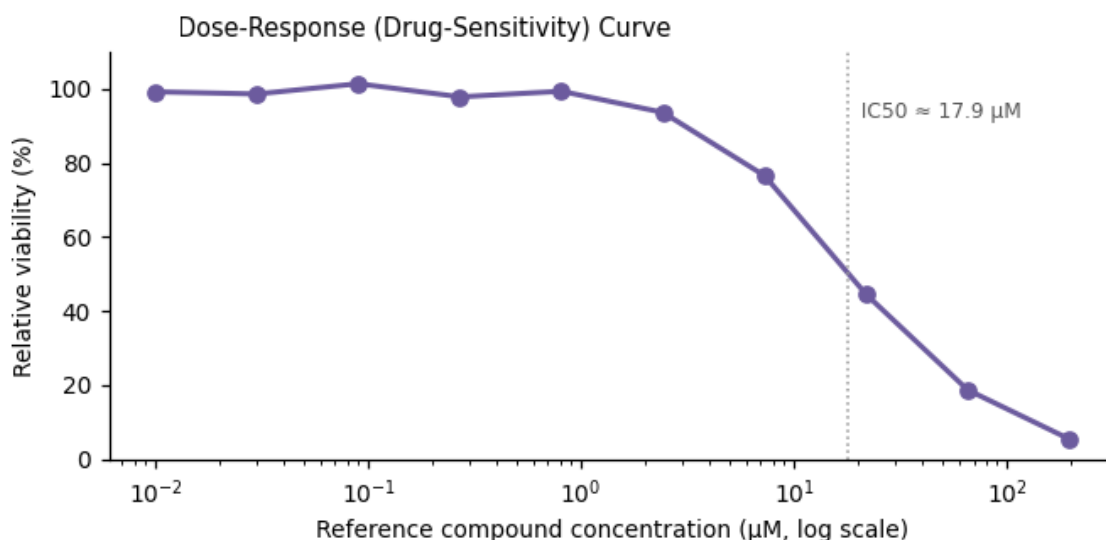
Figure 3. Functional assay readout — IC50 ≈ 17.9 μM.
