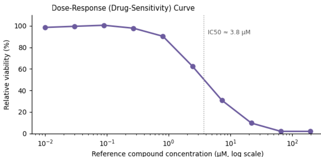
Figure 3. Functional assay readout — IC 50 ≈ 3.8 μM.
