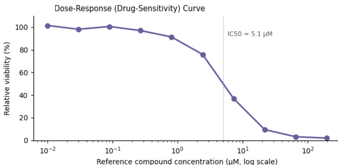
Figure 3. Functional assay readout — IC 50 ≈ 5.1 μM.
