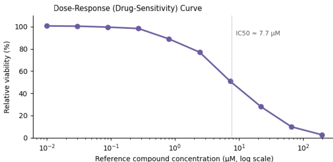
Figure 3. Functional assay readout — IC 50 ≈ 7.7 μM.
