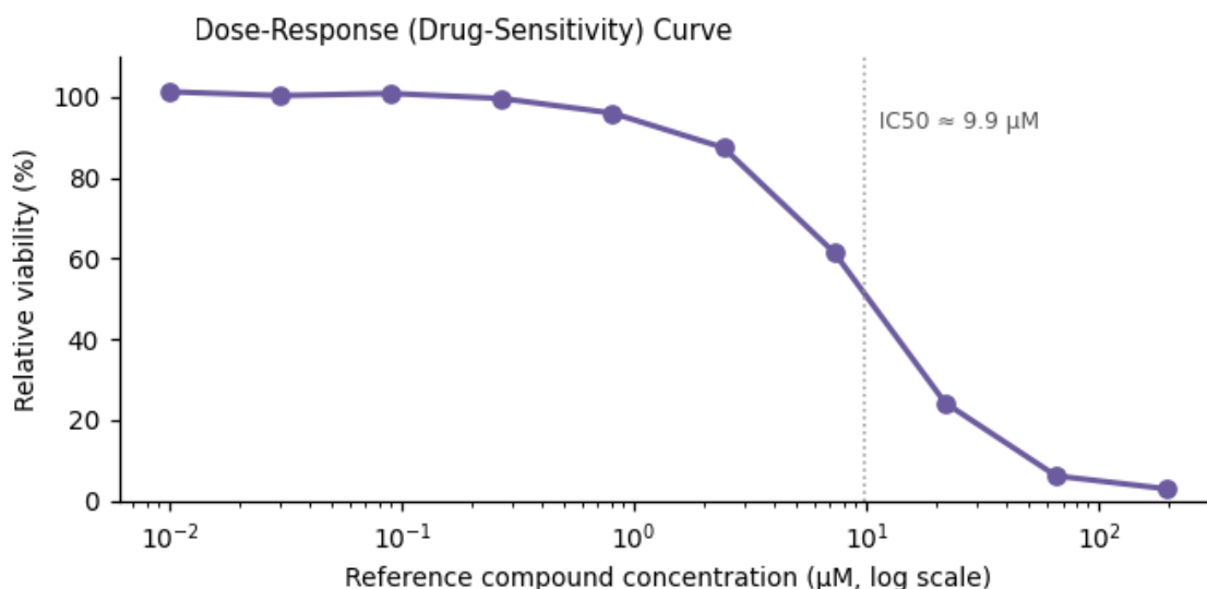
Figure 3. Functional assay readout — IC 50 ≈ 9.9 μM.
