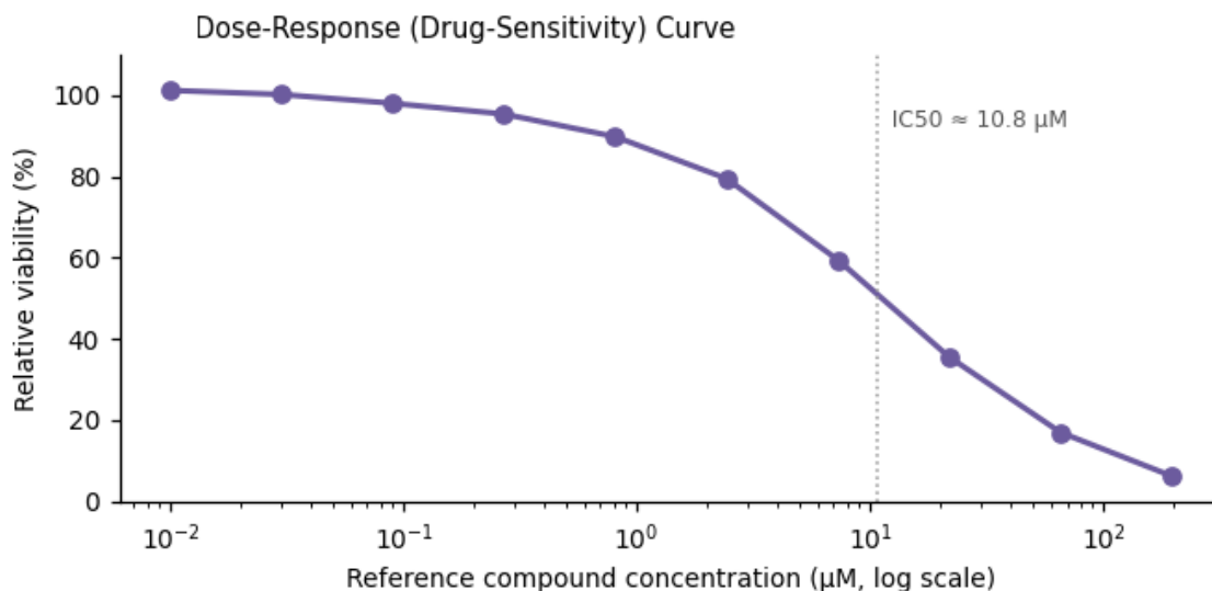
Figure 3. Functional assay readout — IC 50 ≈ 10.8 μM.
