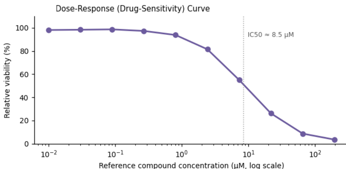
Figure 3. Functional assay readout — IC 50 ≈ 8.5 μM.
