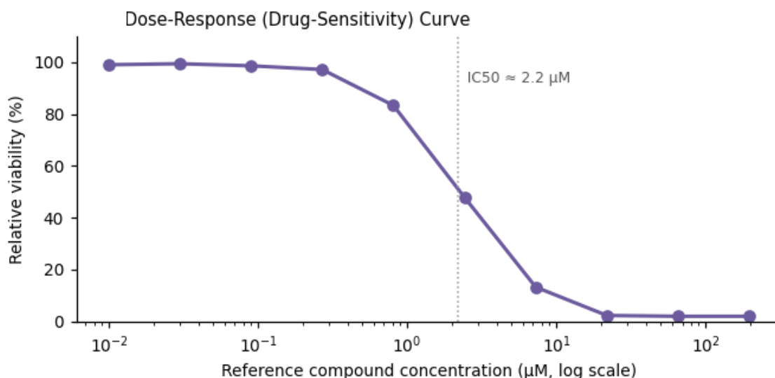
Figure 3. Functional assay readout — IC 50 ≈ 2.2 μM.
