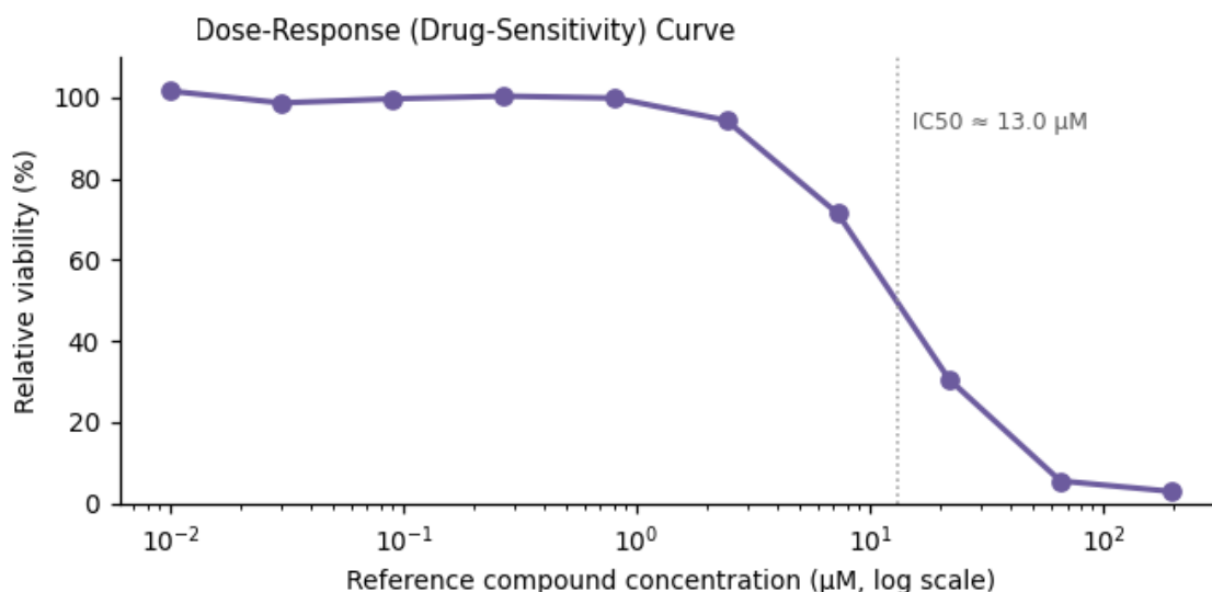
Figure 3. Functional assay readout — IC 50 ≈ 13.0 μM.
