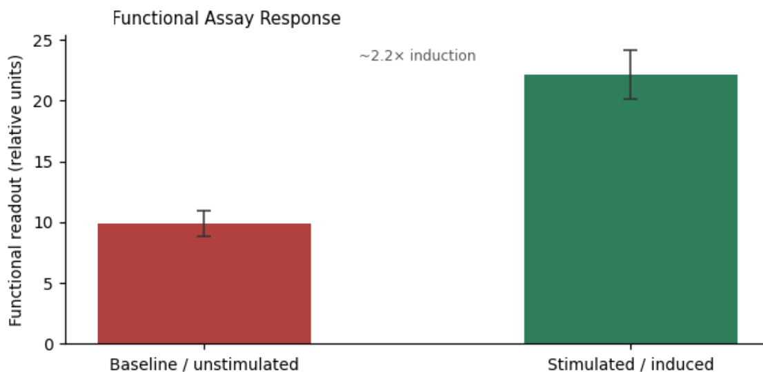
Figure 3. Functional assay readout — ~2.2x induction over baseline.
