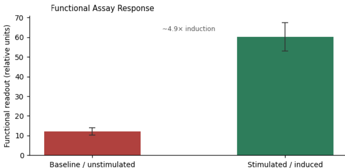
Figure 3. Functional assay readout — ~4.9x induction over baseline.
