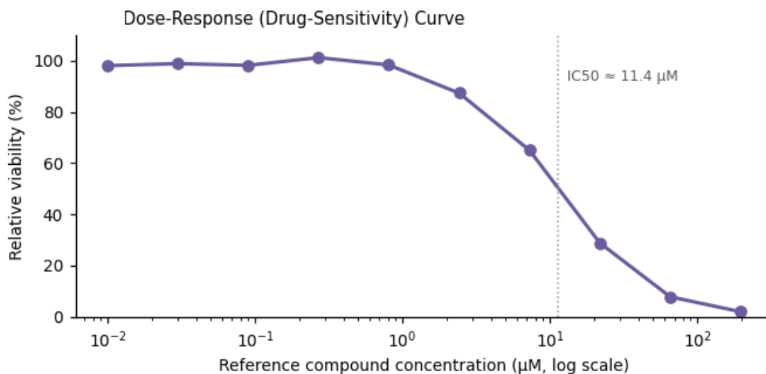
Figure 3. Functional assay readout — IC 50 ≈ 11.4 μM.
