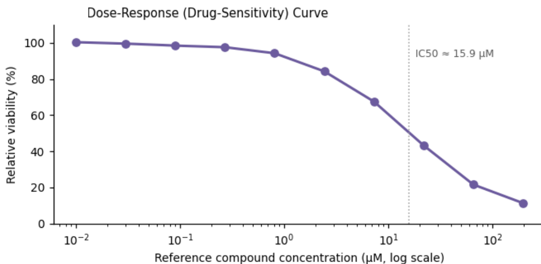
Figure 3. Functional assay readout — \text{IC}_{50} \approx 15.9 \mu\text{M} .
