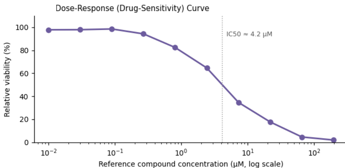
Figure 3. Functional assay readout — IC 50 ≈ 4.2 μM.
