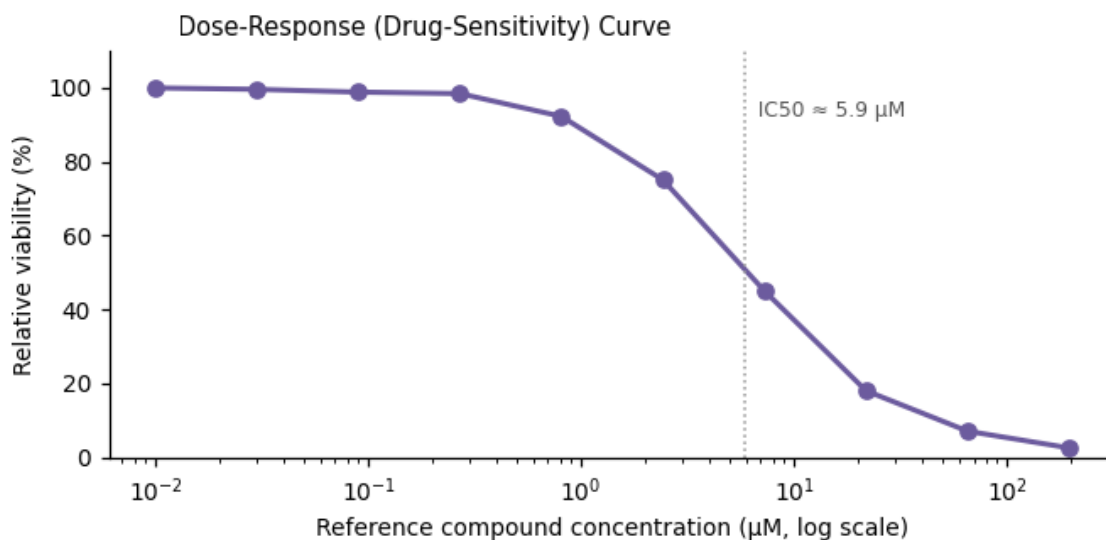
Figure 3. Functional assay readout — IC 50 ≈ 5.9 μM.
