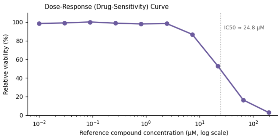
Figure 3. Functional assay readout — \text{IC}_{50} \approx 24.8 \mu\text{M} .
