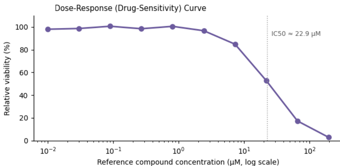
Figure 3. Functional assay readout — \text{IC}_{50} \approx 22.9 \mu\text{M} .
