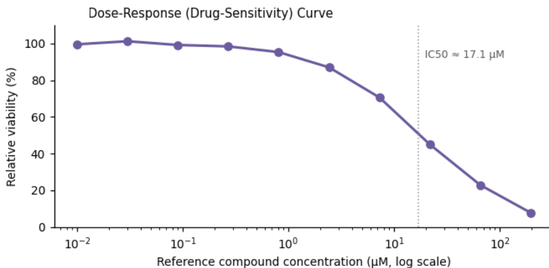
Figure 3. Functional assay readout — \text{IC}_{50} \approx 17.1 \mu\text{M} .
