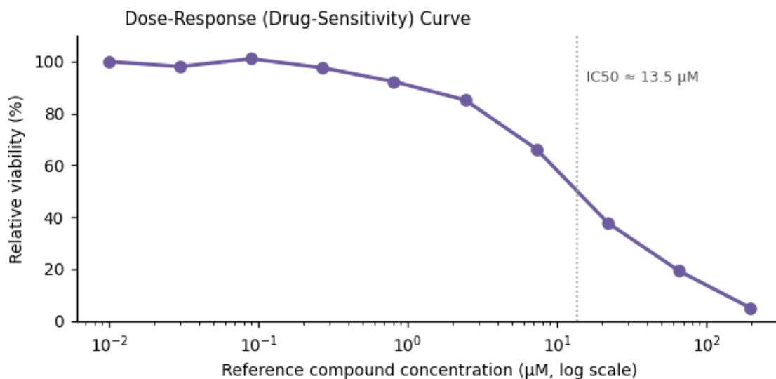
Figure 3. Functional assay readout — \text{IC}_{50} \approx 13.5 \mu\text{M} .
