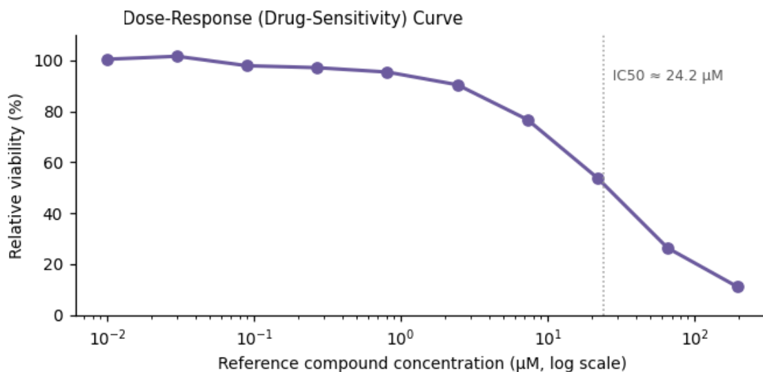
Figure 3. Functional assay readout — \text{IC}_{50} \approx 24.2 \mu\text{M} .
