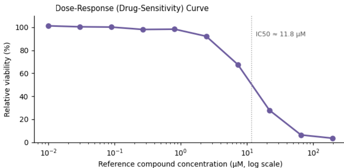
Figure 3. Functional assay readout — IC 50 ≈ 11.8 μM.
