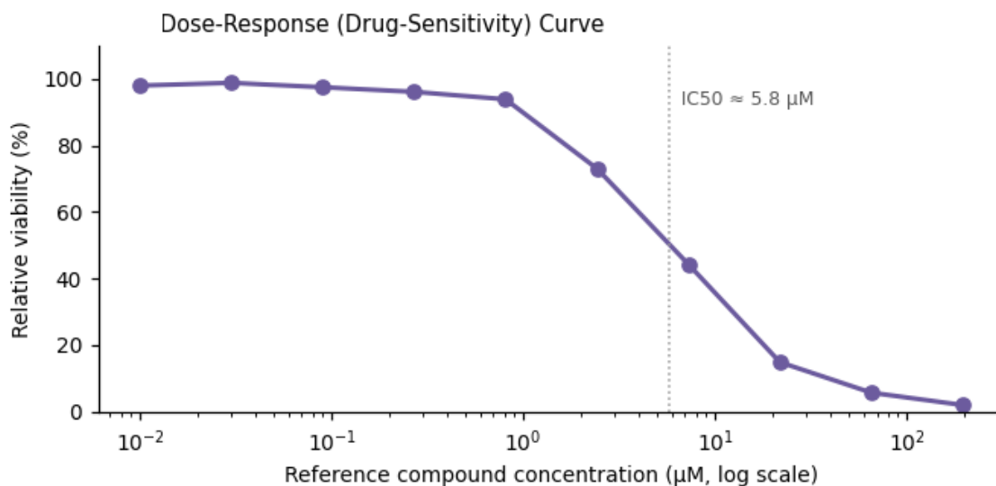
Figure 3. Functional assay readout — IC 50 ≈ 5.8 µM.
