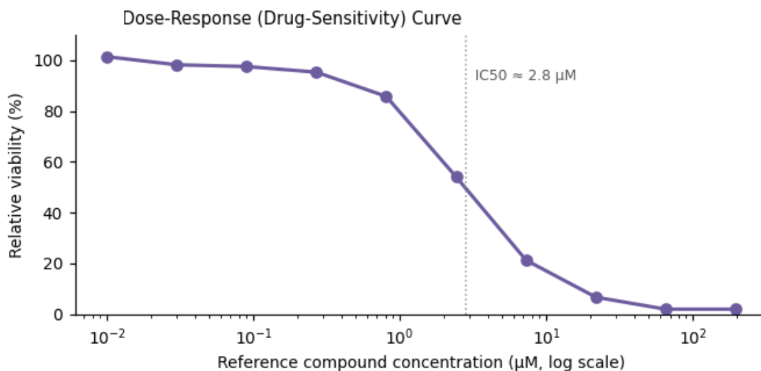
Figure 3. Functional assay readout — \text{IC}_{50} \approx 2.8 \mu\text{M} .
