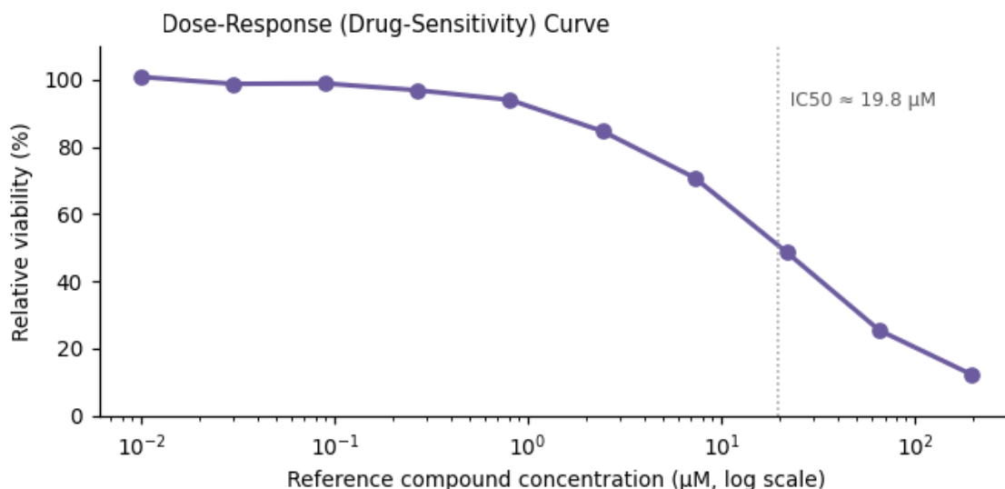
Figure 3. Functional assay readout — \text{IC}_{50} \approx 19.8 \mu\text{M} .
