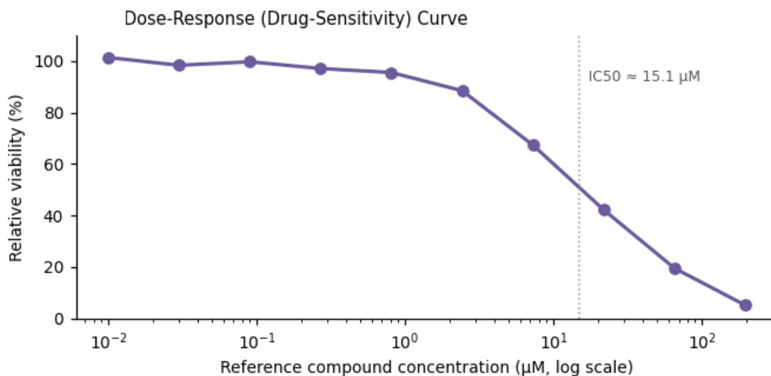
Figure 3. Functional assay readout — IC 50 ≈ 15.1 µM.
