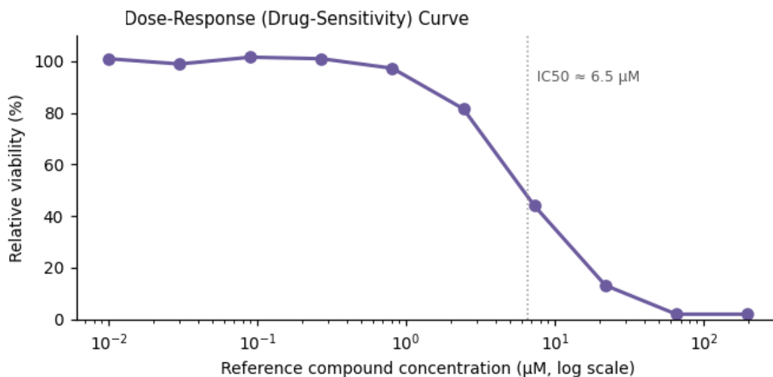
Figure 3. Functional assay readout — IC 50 ≈ 6.5 µM.
