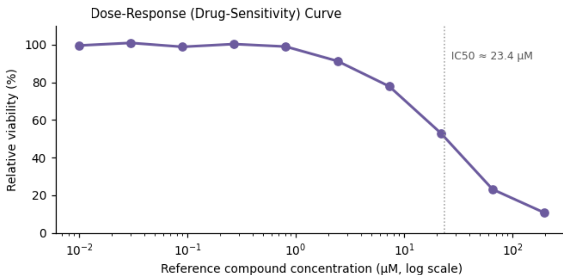
Figure 3. Functional assay readout — IC 50 ≈ 23.4 μM.
