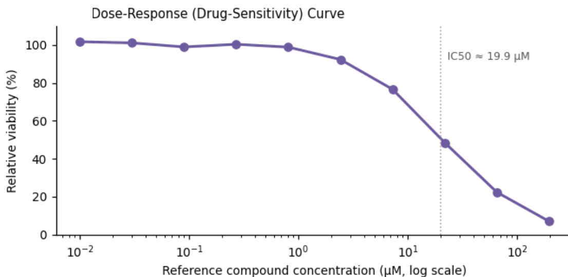
Figure 3. Functional assay readout — \text{IC}_{50} \approx 19.9 \mu\text{M} .
