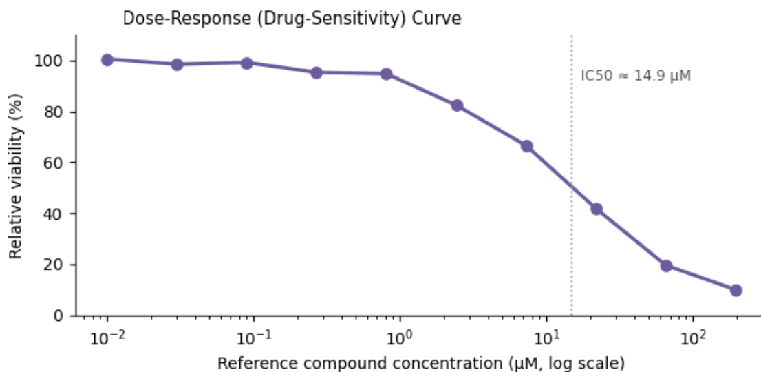
Figure 3. Functional assay readout — \text{IC}_{50} \approx 14.9 \mu\text{M} .
