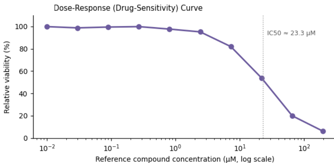
Figure 3. Functional assay readout — IC 50 ≈ 23.3 μM.
