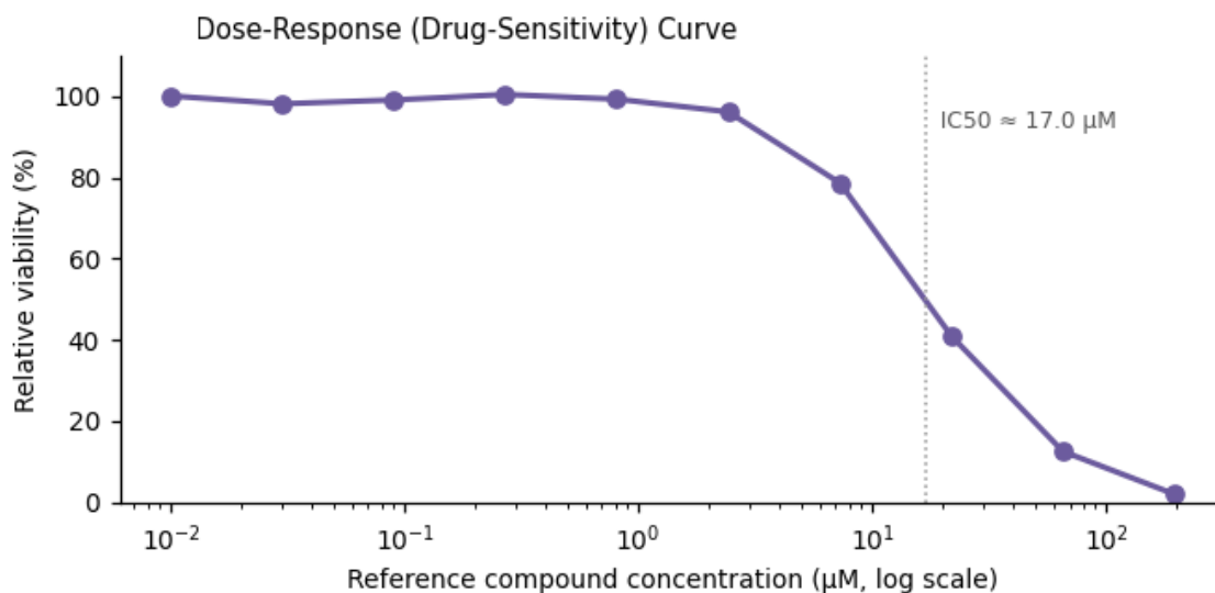
Figure 3. Functional assay readout — IC 50 ≈ 17.0 μM.
