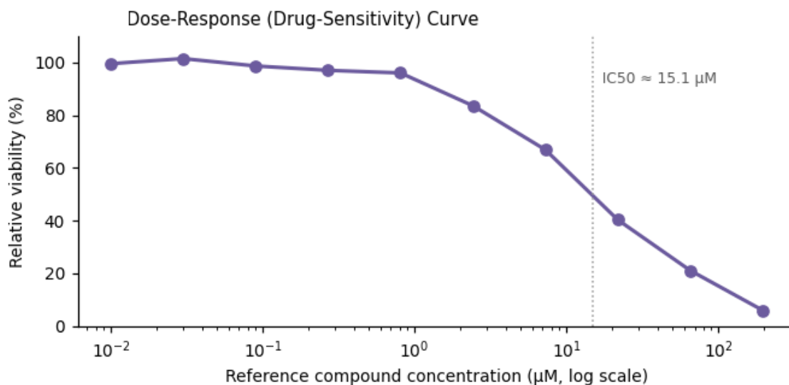
Figure 3. Functional assay readout — \text{IC}_{50} \approx 15.1 \mu\text{M} .
