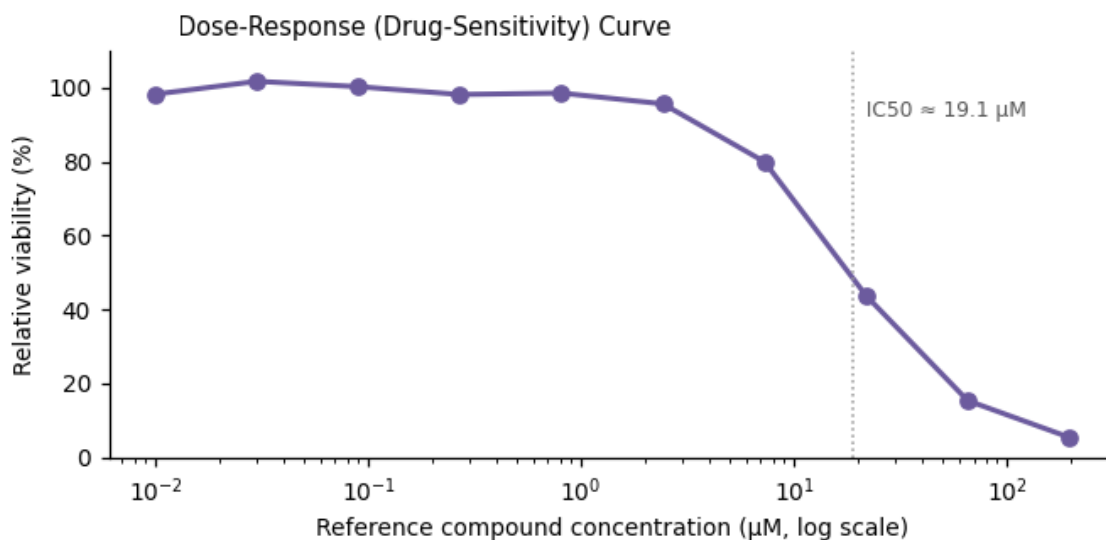
Figure 3. Functional assay readout — IC 50 ≈ 19.1 μM.
