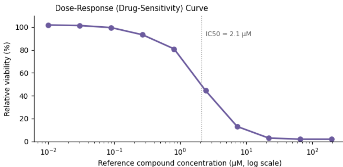
Figure 3. Functional assay readout — \text{IC}_{50} \approx 2.1 \mu\text{M} .
