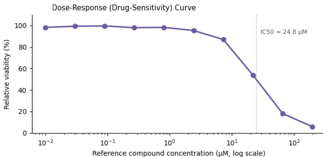
Figure 3. Functional assay readout — IC 50 ≈ 24.8 μM.
