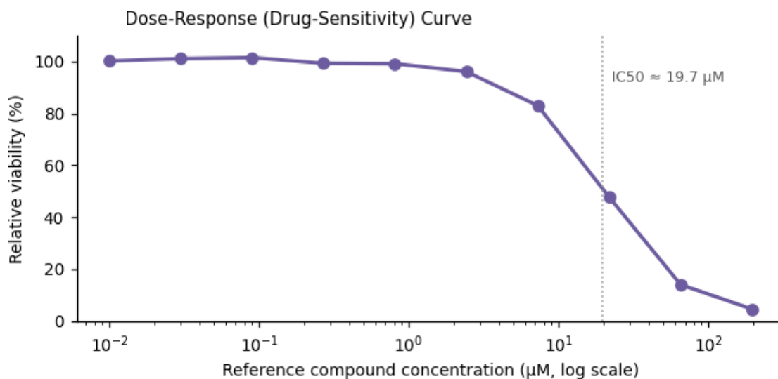
Figure 3. Functional assay readout — IC 50 ≈ 19.7 μM.
