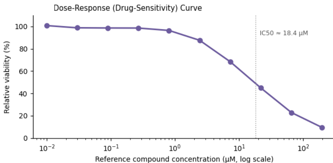
Figure 3. Functional assay readout — \text{IC}_{50} \approx 18.4 \mu\text{M} .
