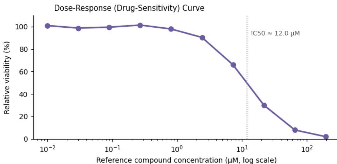
Figure 3. Functional assay readout — IC 50 ≈ 12.0 μM.
