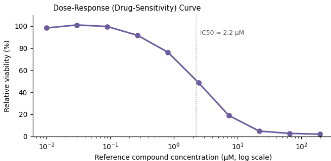
Figure 3. Functional assay readout — \text{IC}_{50} \approx 2.2 \mu\text{M} .
