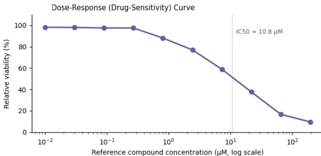
Figure 3. Functional assay readout — \text{IC}_{50} \approx 10.8 \mu\text{M} .
